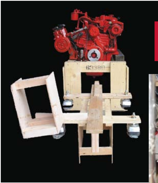
From top: the engine mockup, necessary hardware, hoses. Below, hoses clamped on the clean bilge. Opposite: top, trial fit of engine in new bed; bottom, front view of the compressor mount
